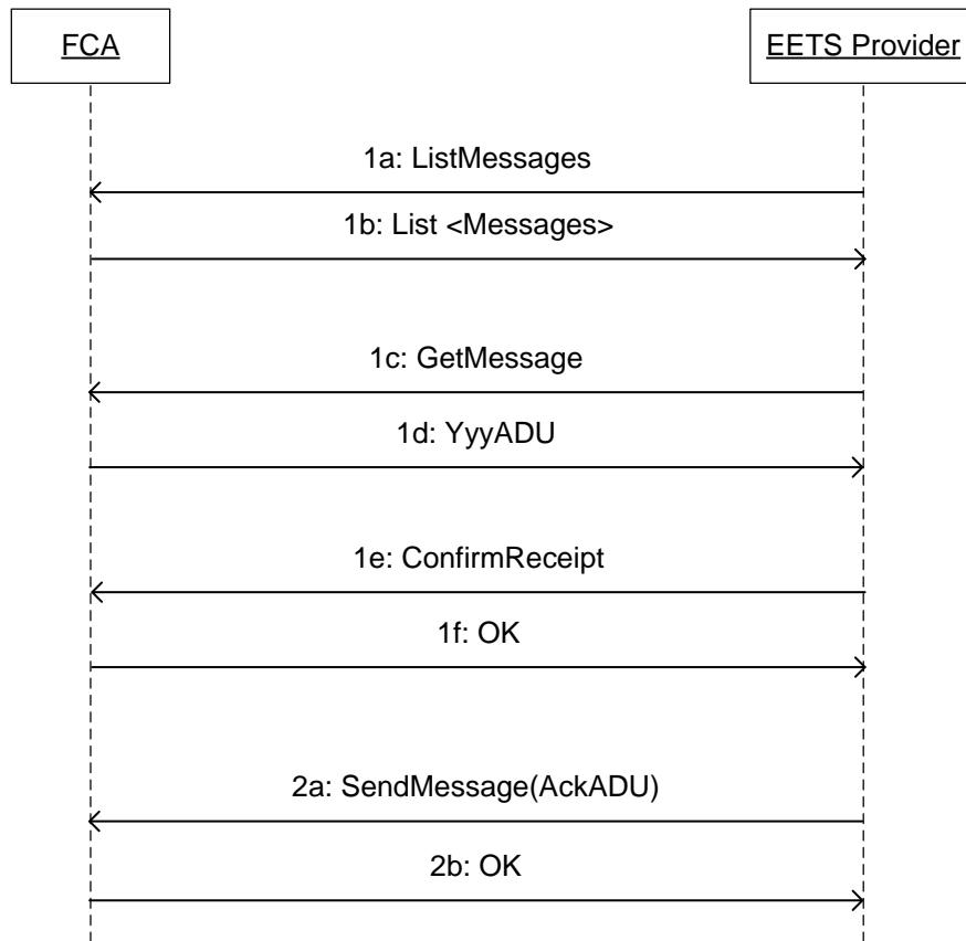
Figure 6 – FCA to EETS provider transport layer protocol
