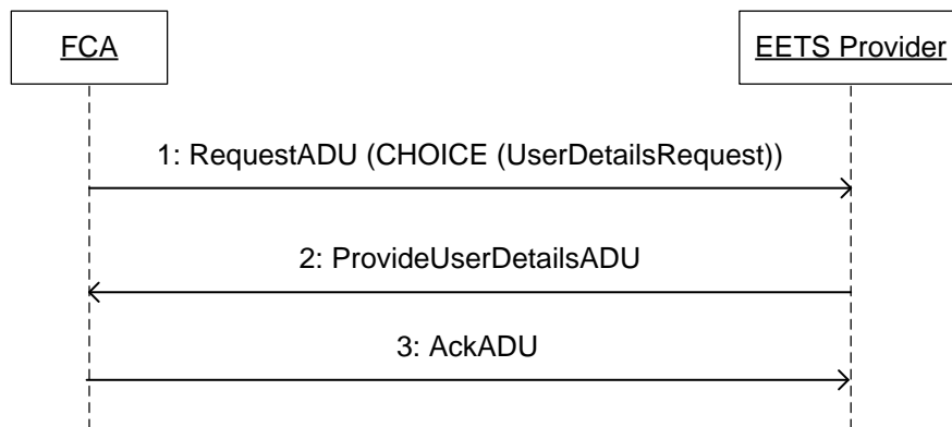
Figure 7 – Request messages from FCA to EETS provider
