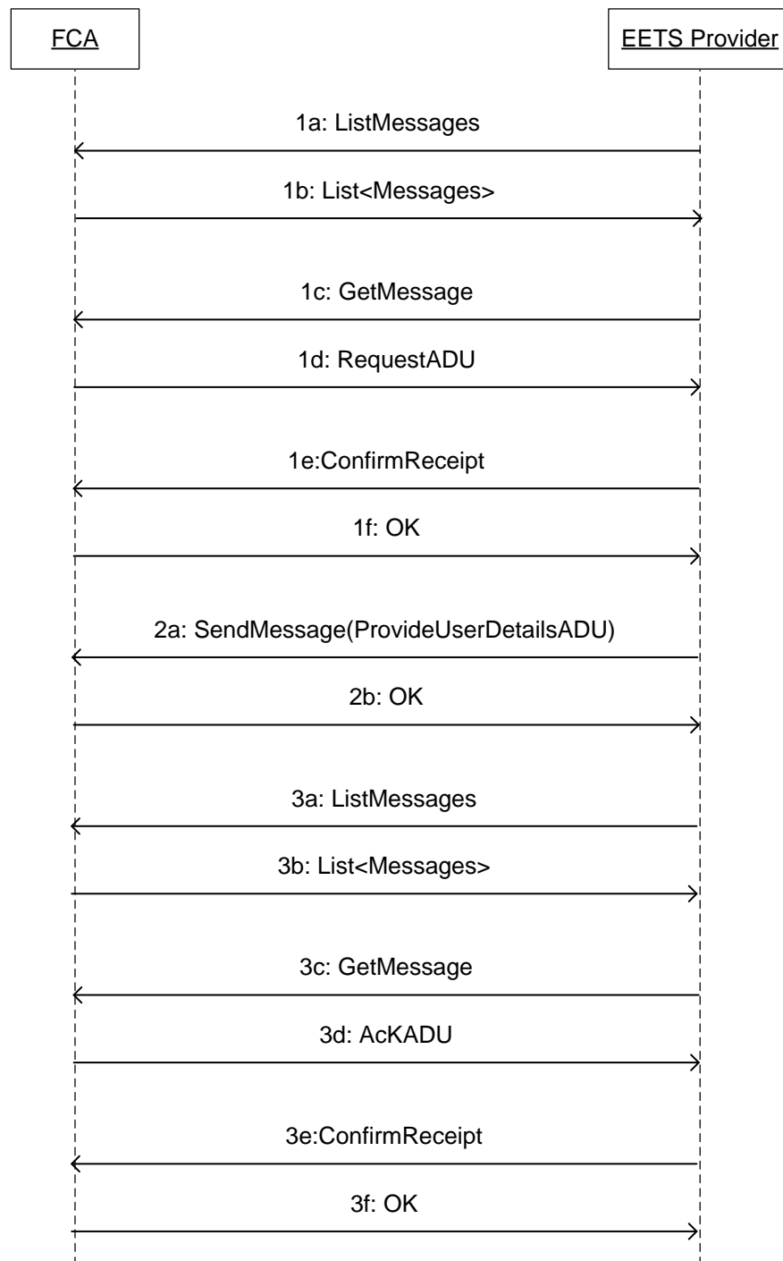
Figure 8 – FCA to EETS provider request message transport layer protocol
