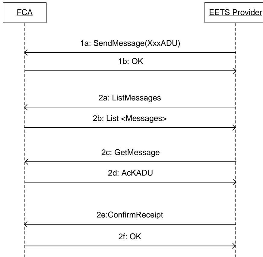
Figure 4 – EETS provider to FCA transport layer protocol
