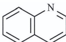
Chinolin
